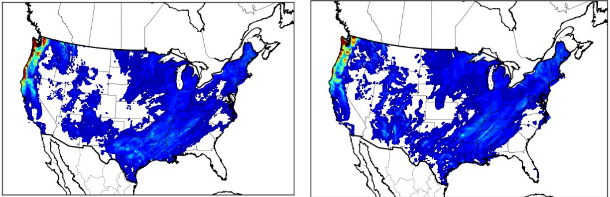
PRISM, November 2016
