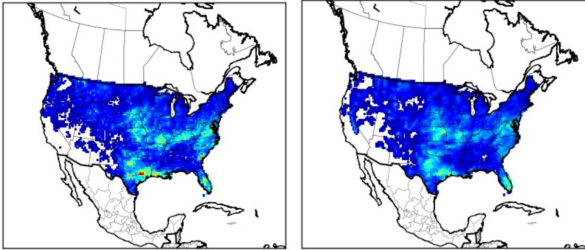
PRISM, May 2016
