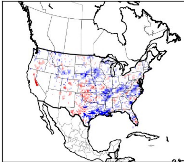
WRF - Prism, May 2016
