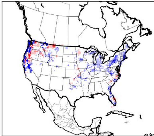
WRF - Prism, October 2016
