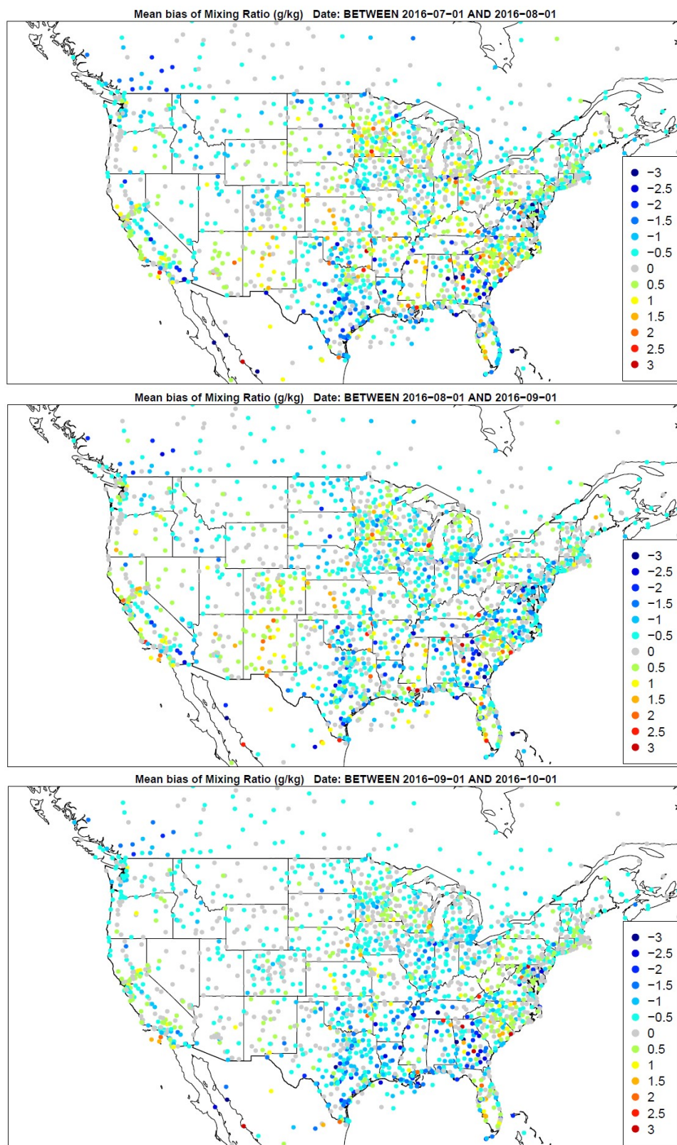
Figure 3.3.17. Spatial distribution of water vapor mixing ratio bias (g/kg) across daytime hours for the months of July, August, and September (top to bottom) for the 12US domain.
