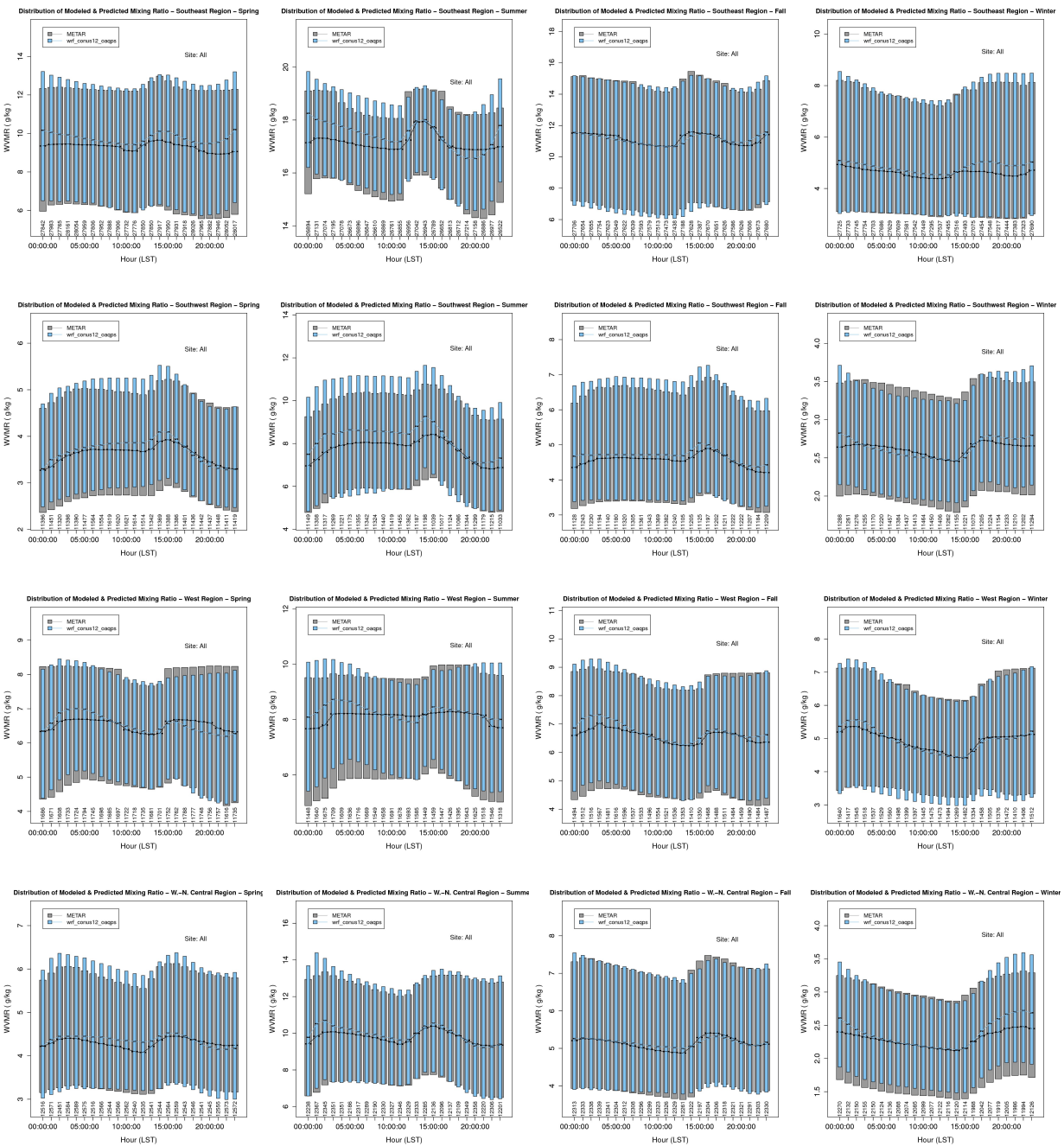
Figure 3.3.19. Hourly average distribution of observed and predicted water vapor mixing ratio for the 12US domain in the Central, East-North Central, Northeast, Northwest, South, Southeast, Southwest, West, and West-North Central (top to bottom) regions for each season (Spring, Summer, Fall, Winter, L-R).
