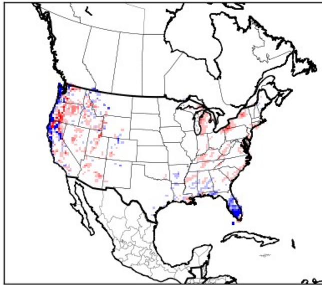
WRF - Prism, January 2016
