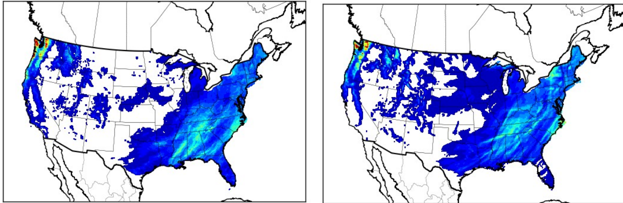
WRF, February 2016
