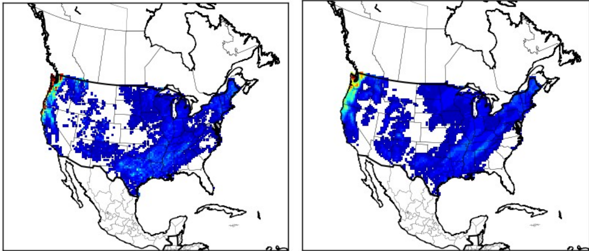
PRISM, November 2016
