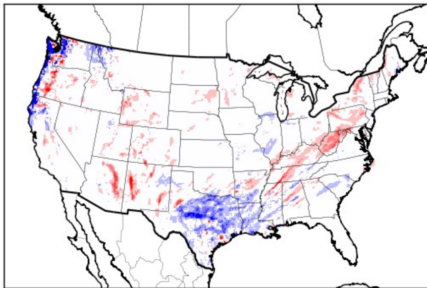
WRF - PRISM, November 2016
