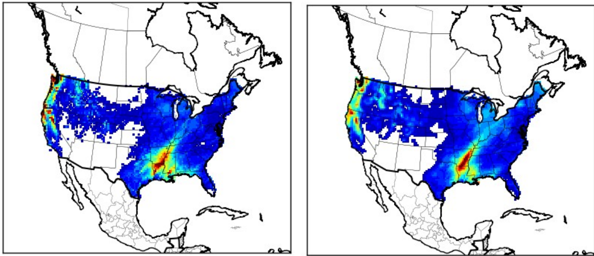
WRF, March 2016
