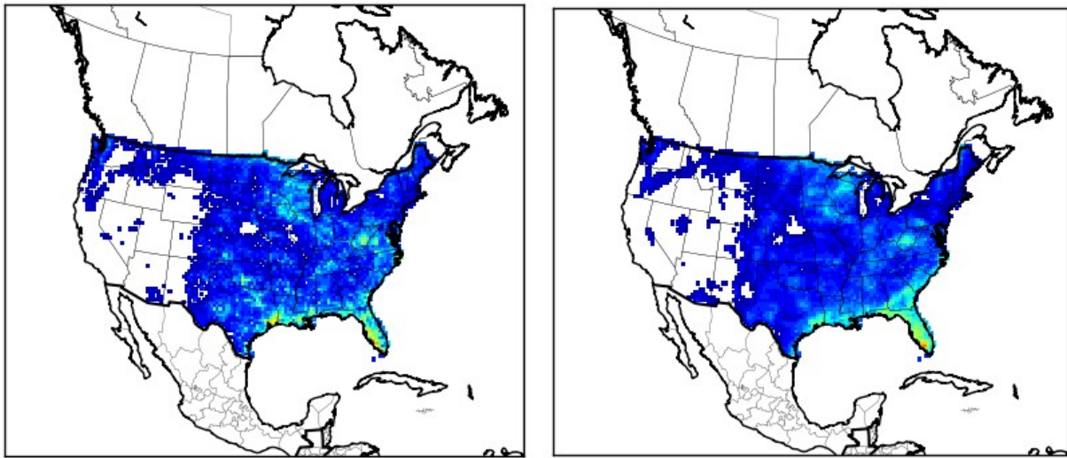
WRF, June 2016
