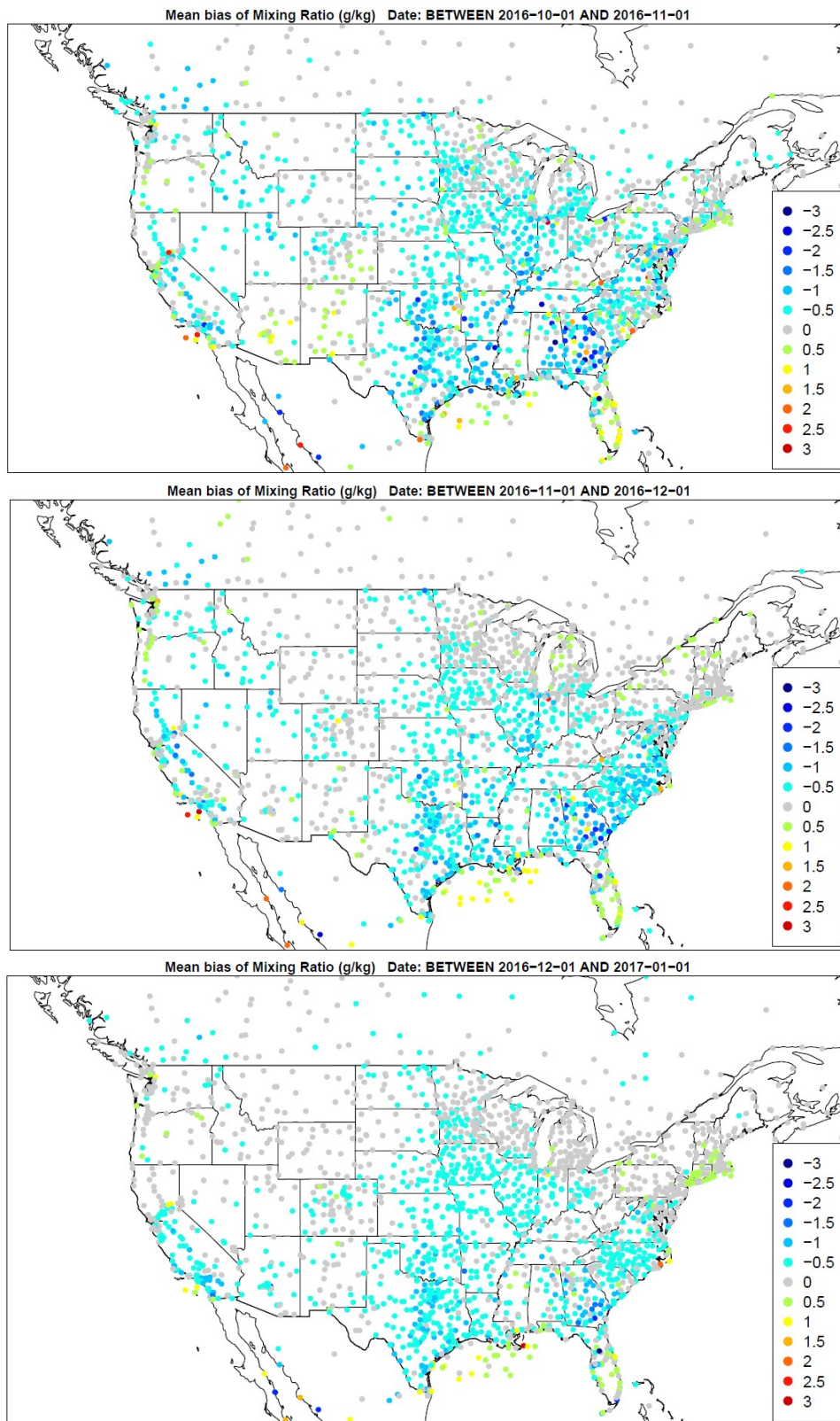
Figure 3.3.10. Spatial distribution of water vapor mixing ratio bias (g/kg) across all hours for the months of October, November, and December (top to bottom) for the 12US domain.
