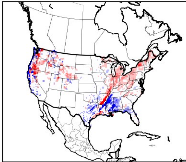
WRF - Prism, March 2016
