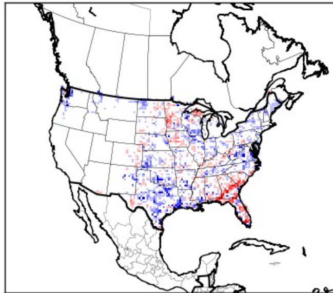
WRF - Prism, June 2016
