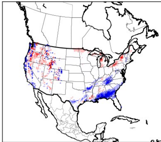
WRF - Prism, December 2016
