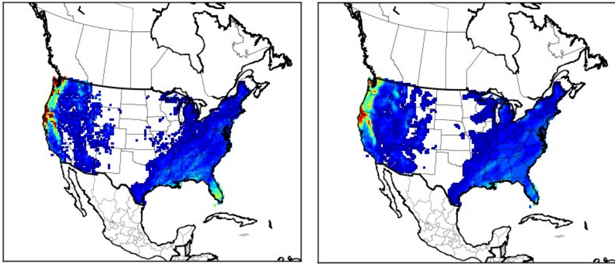
PRISM, January 2016
