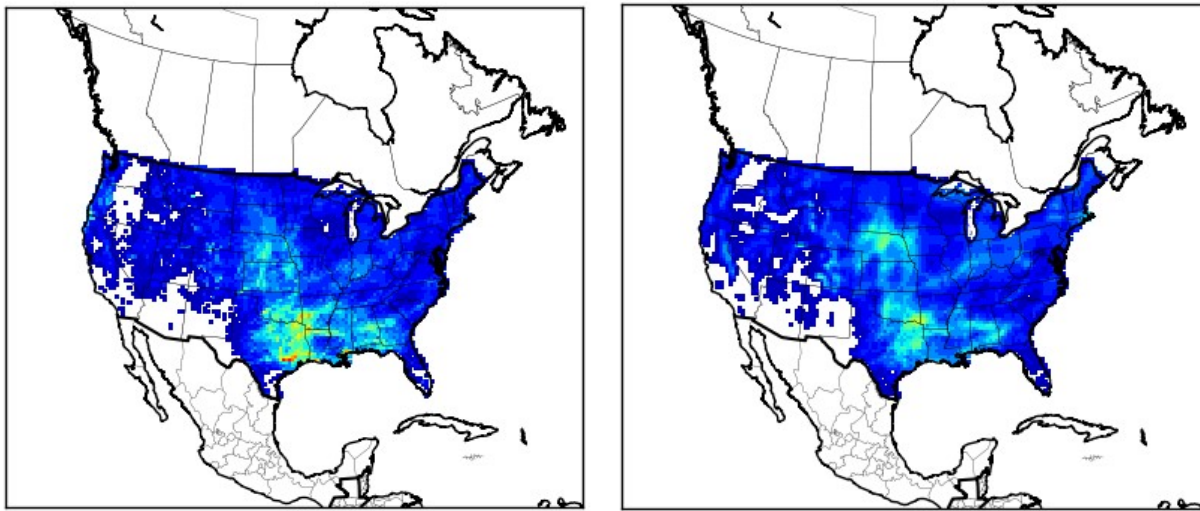
PRISM, April 2016
