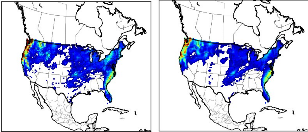
PRISM, October 2016
