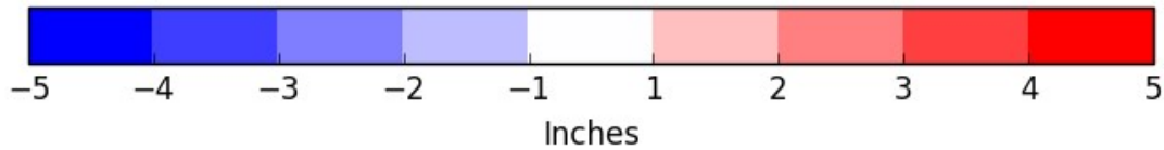
Figure 3.4.1. PRISM analysis (top left) and WRF (top right) estimated monthly total rainfall (in) and the difference (bottom) for January for the 36NOAM simulation.
