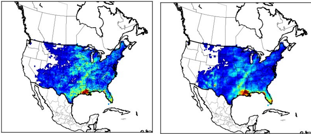
WRF, August 2016
