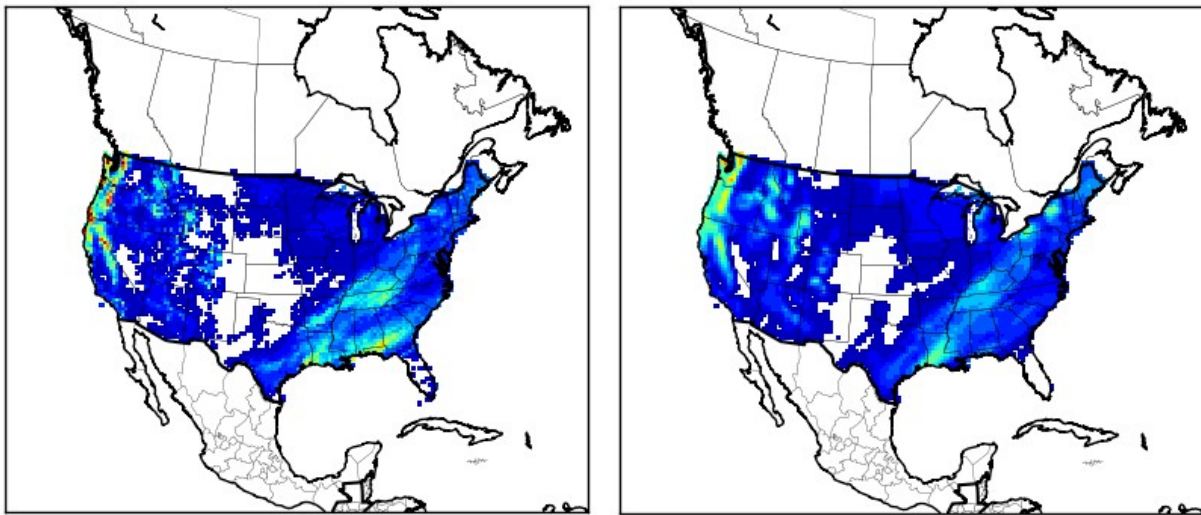
PRISM, December 2016
