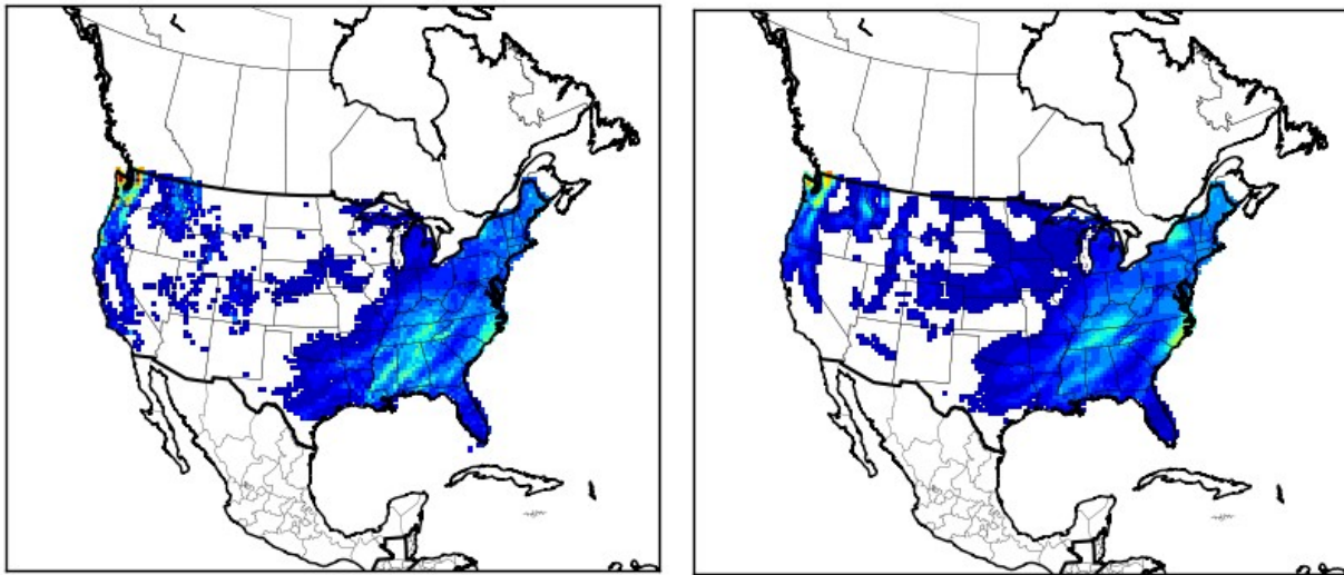
WRF, February 2016
