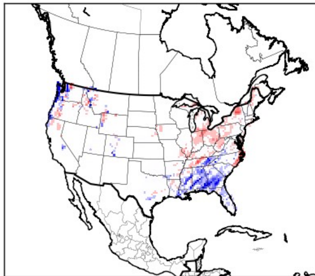
WRF - Prism, February 2016
