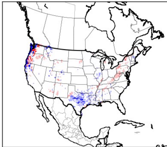
WRF - Prism, November 2016
