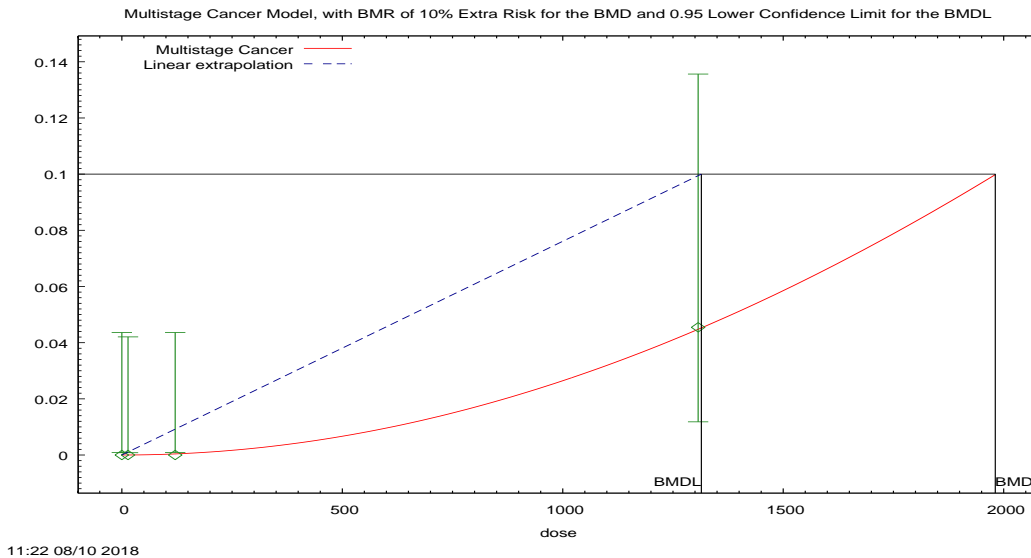
Figure K-22. Plot of incidence rate by dose with fitted curve for Multistage-Cancer 2° model for Nasal cavity tumors in Sherman rats Kociba et al. (1974) ; dose shown in mg/kg-d.
