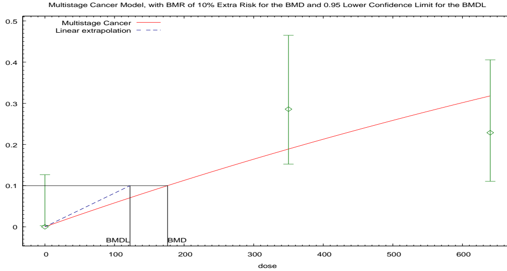
Figure K-24. Plot of incidence rate by dose with fitted curve for Multistage-Cancer 1° model for Nasal squamous cell carcinomas in female OM rats (MS models) NCI (1978) ; dose shown in mg/kg-d.
