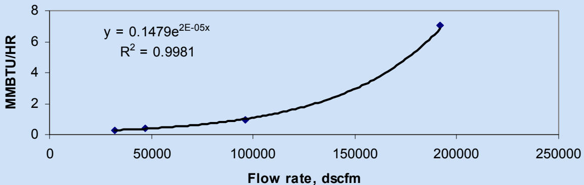
Figure 3-3. Relationship between RTO natural gas consumption and flow rate.
