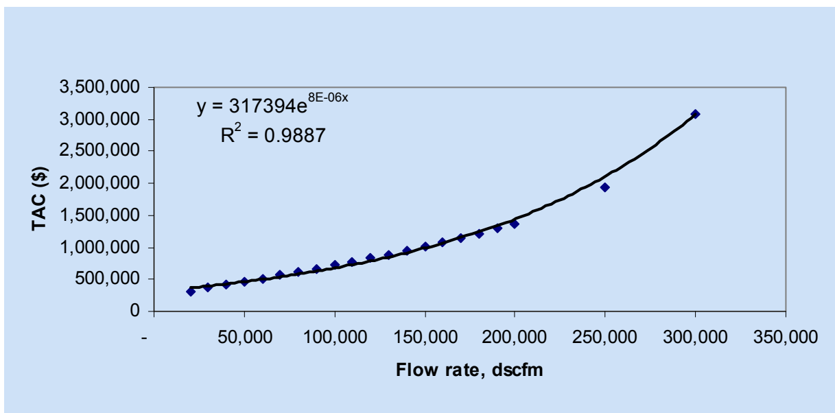
Figure 3-5. Variation in RTO total annualized cost with flow.
