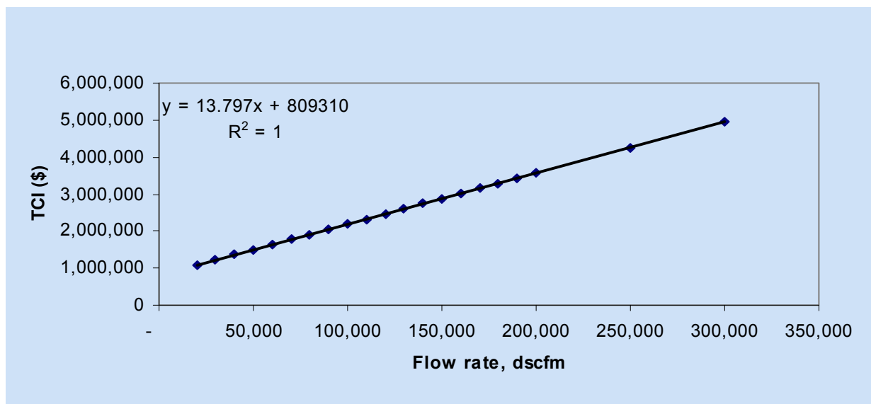
Figure 3-4. Variation in RTO total capital investment with flow.
