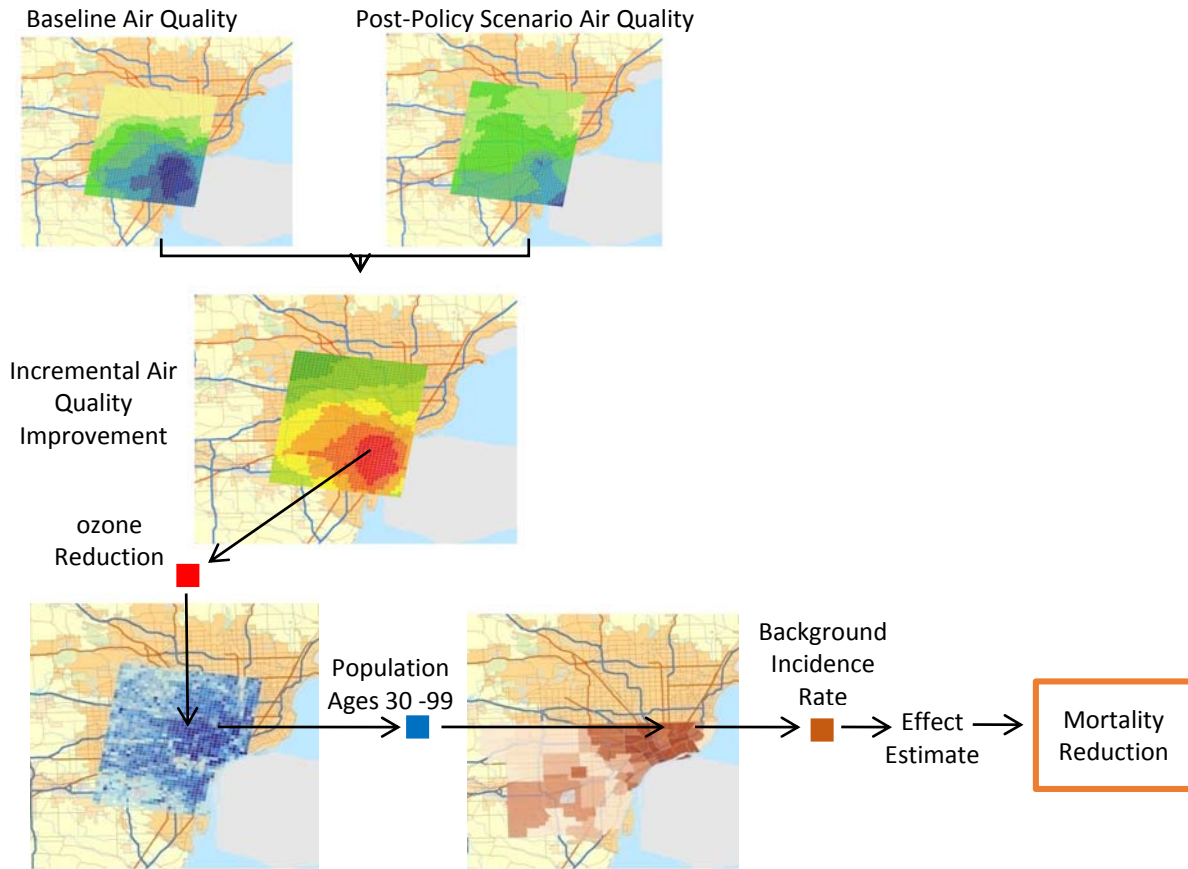
Figure 5-1. Illustration of BenMAP-CE Approach
