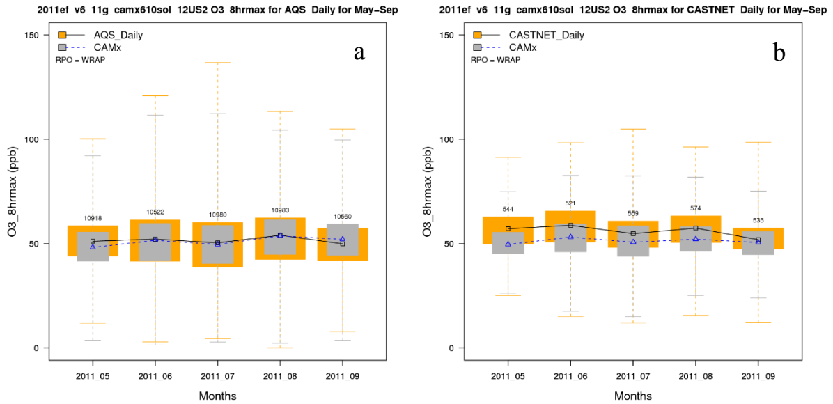
Figure 3A-5. Distribution of observed and predicted MDA8 ozone by month for the period May through September for the West, (a) AQS network and (b) CASTNet network
