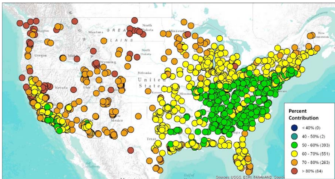
Figure 2-9. Map of Site-Specific Ratios of U.S. Background to Total Seasonal Mean Ozone based on 2007 CMAQ Zero-Out Modeling
