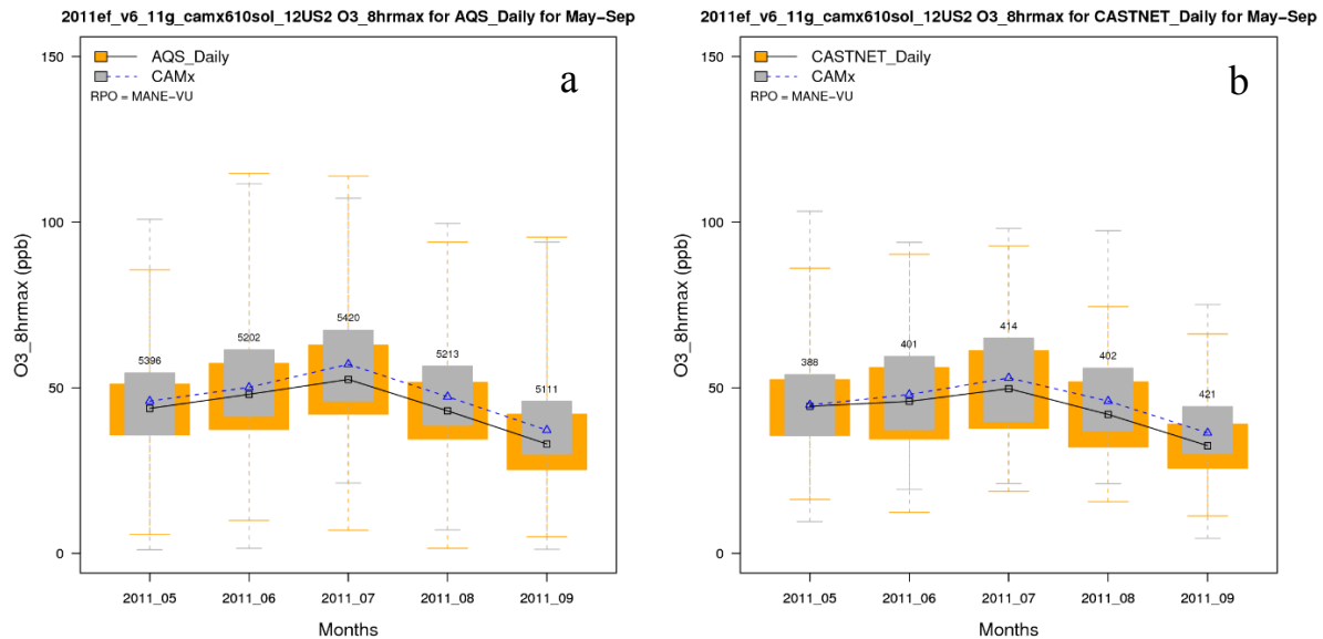
Figure 3A-1. Distribution of observed and predicted MDA8 ozone by month for the period May through September for the Northeast subregion, (a) AQS network and (b) CASTNet network. [symbol = median; top/bottom of box = 75th/25th percentiles; top/bottom line = max/min values]
