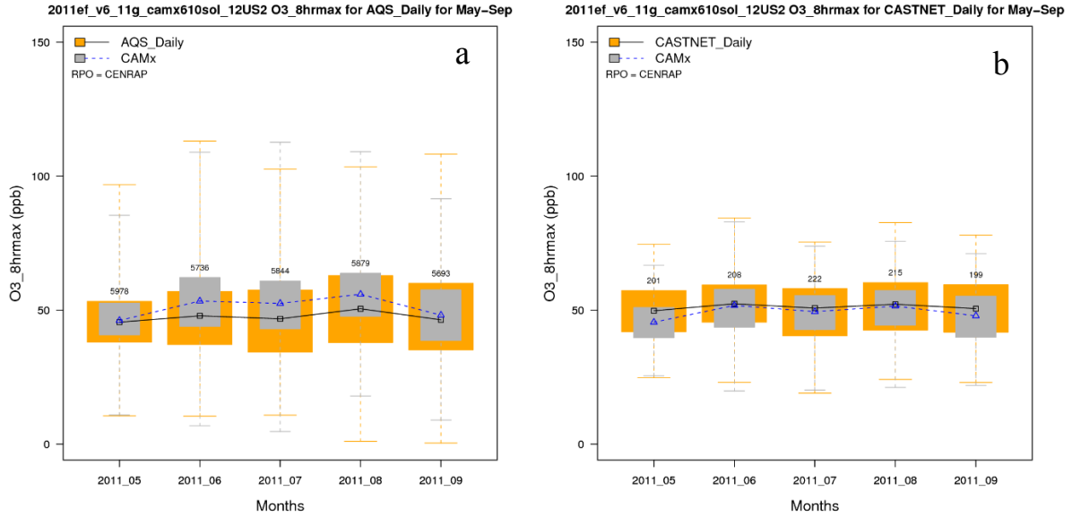
Figure 3A-4. Distribution of observed and predicted MDA8 ozone by month for the period May through September for the Central states, (a) AQS network and (b) CASTNet network
