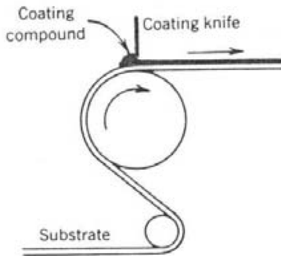
Figure 2-3. Knife-Over-Roll Coating
