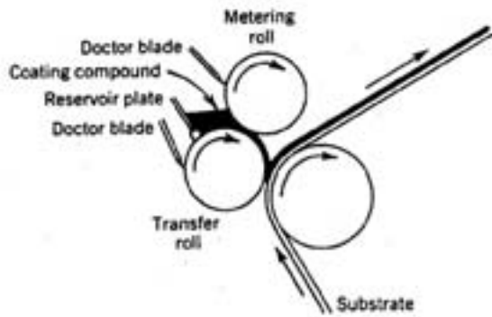
Figure 2-4. Reverse-Roll Coating
