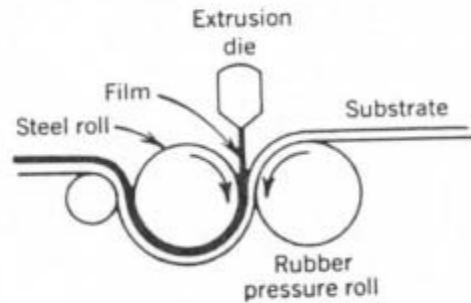
Figure 2-7. Extrusion Coating
