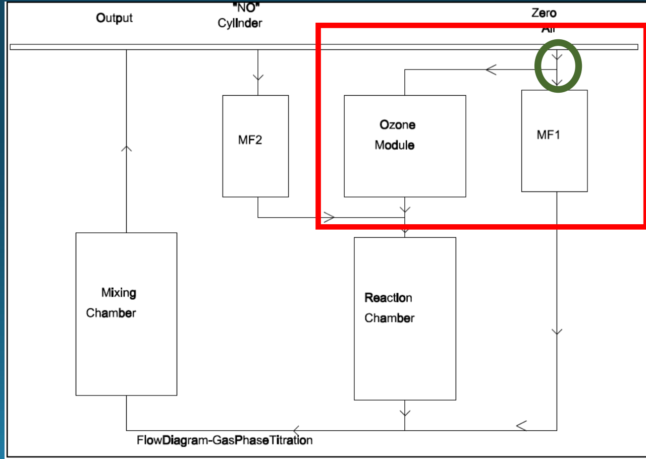
Caution- pre MFC bypass for O 3
