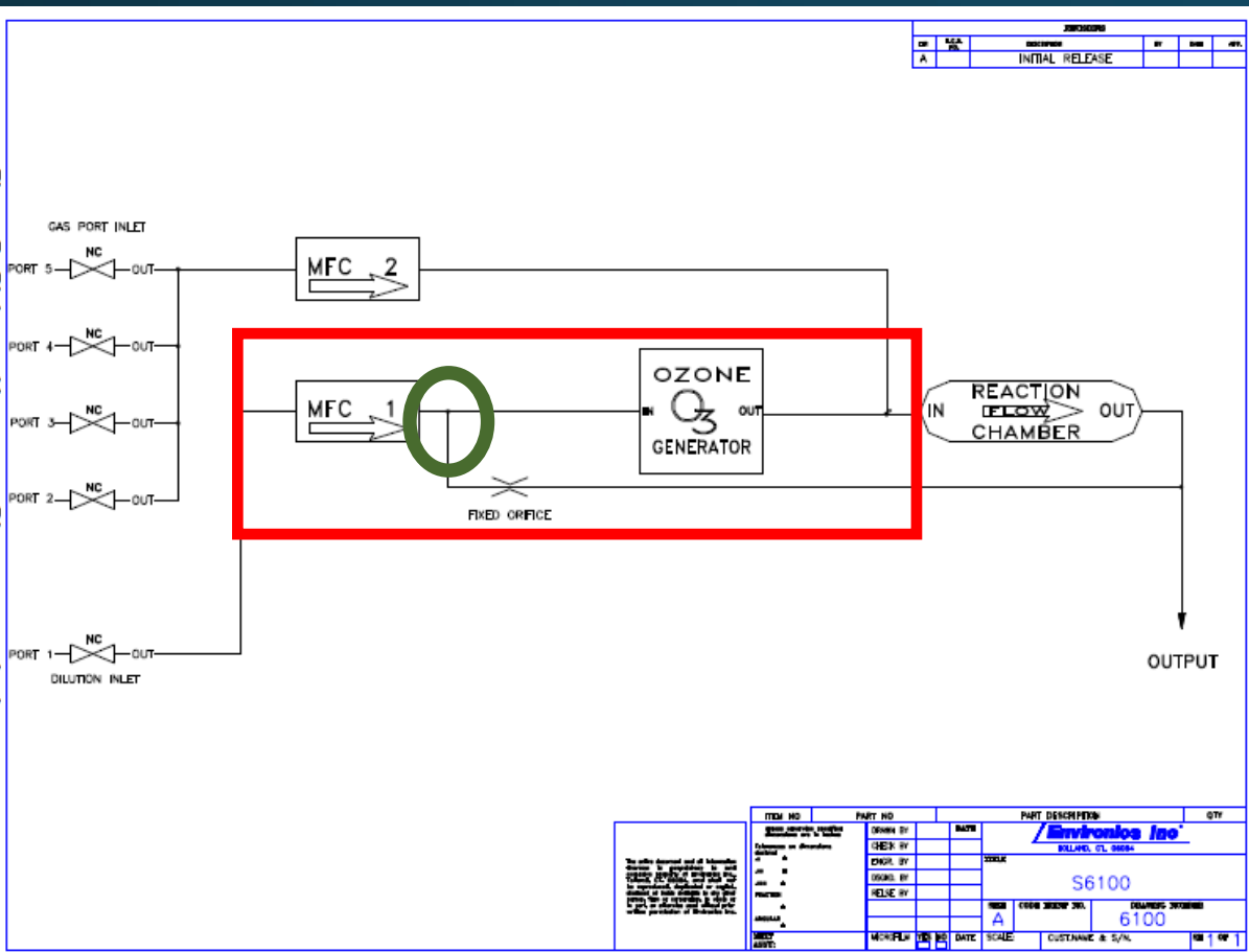
Simple Setup/post MFC bypass for O 3
